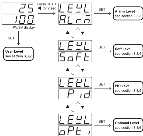
Figure 5. Menu flowchart
