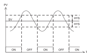
Figure 11. ON/OFF Control Action
