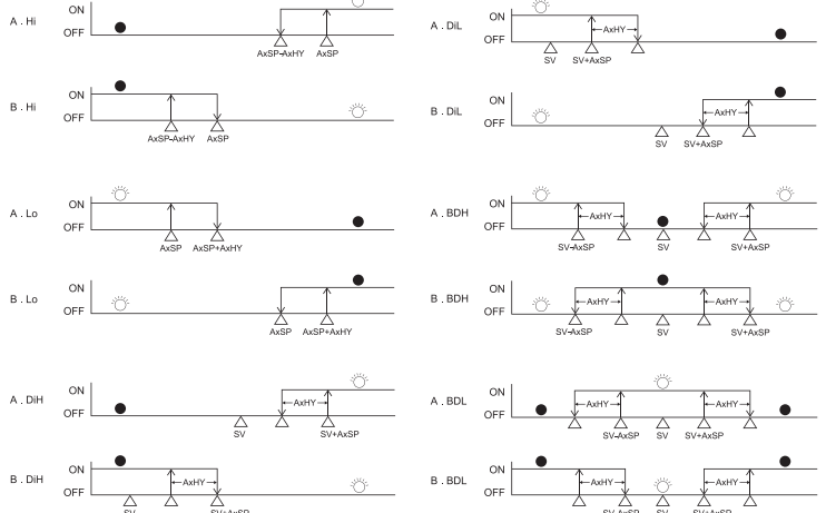
Figure 7. Alarm function
