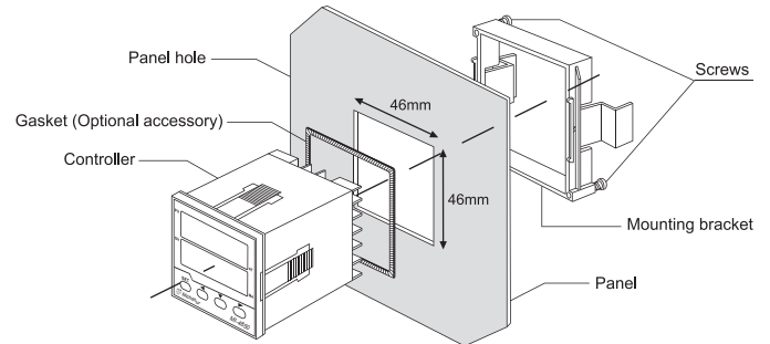
Figure 1. Panel mounting
