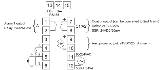
Figure 2. Terminal connections
