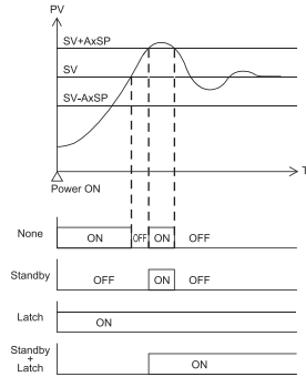
Figure 8. Alarm Mode
